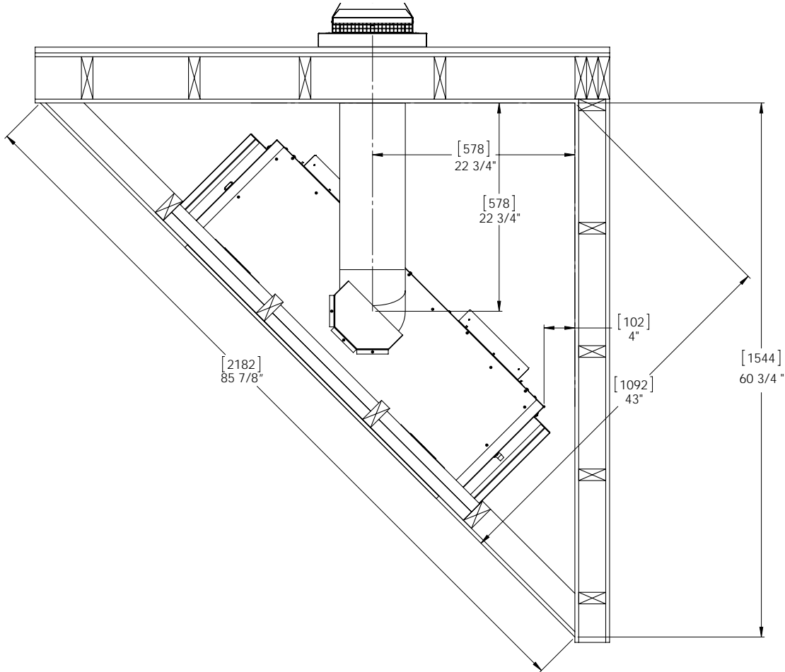
Figure 48: Dimensions for a Corner Installation
