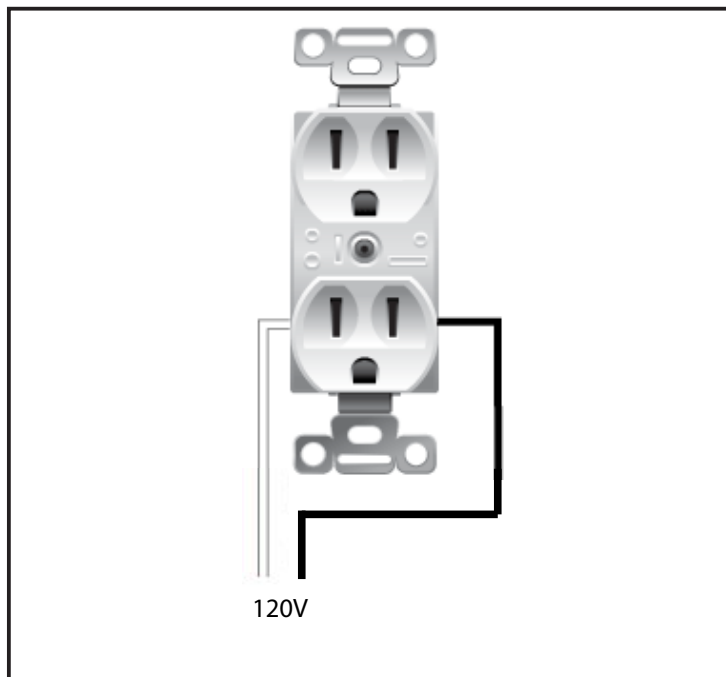
Figure 68: C34I Receptacle Wiring
