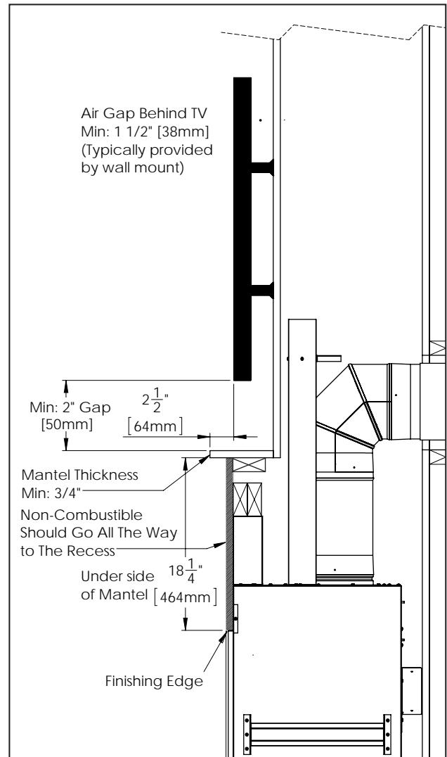
Figure 53: Recess Minimum TV Install Clearances
