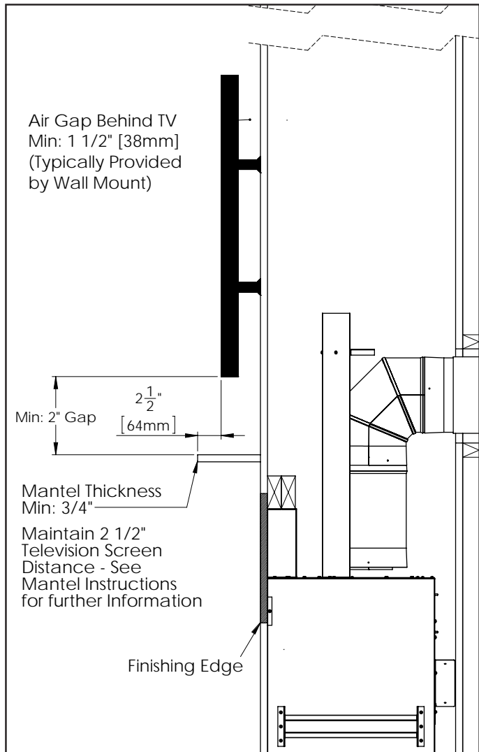
Figure 52: Minimum TV Install Clearances
