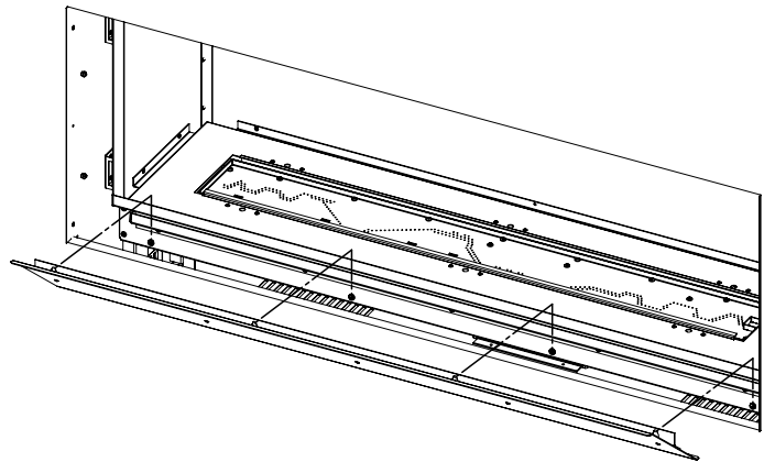
Figure 8: Removing Intake Shield
