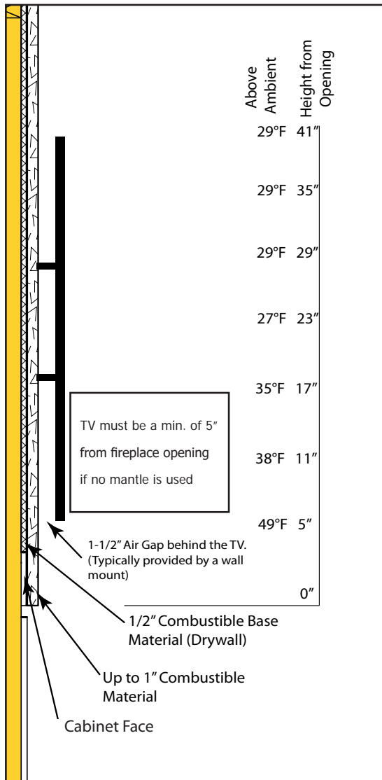
Figure 39: CSS TV Clearances
