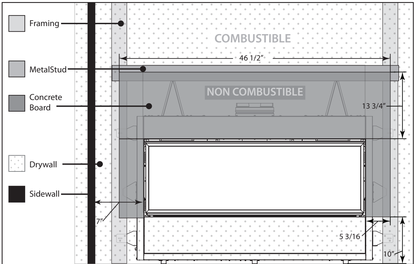
Figure 30: Non-Combustible Zones
