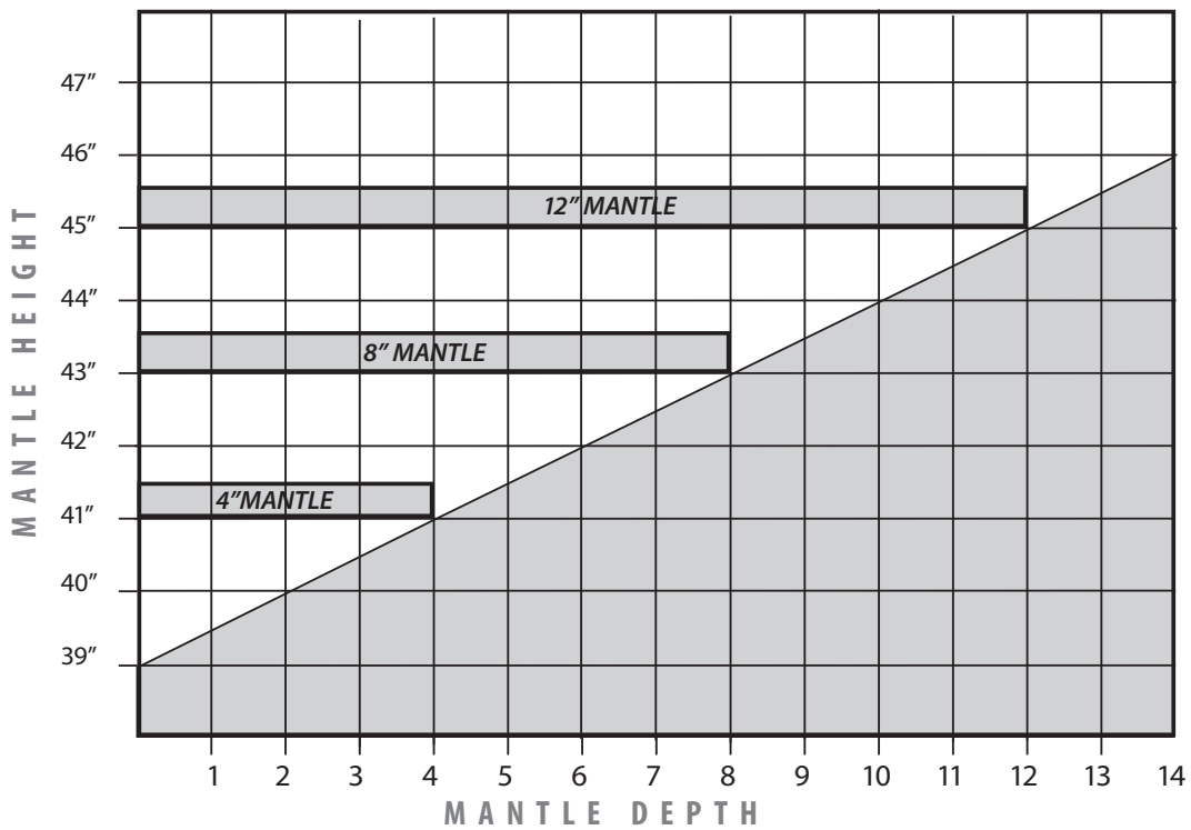
Figure 44: Minimum Mantel Height
