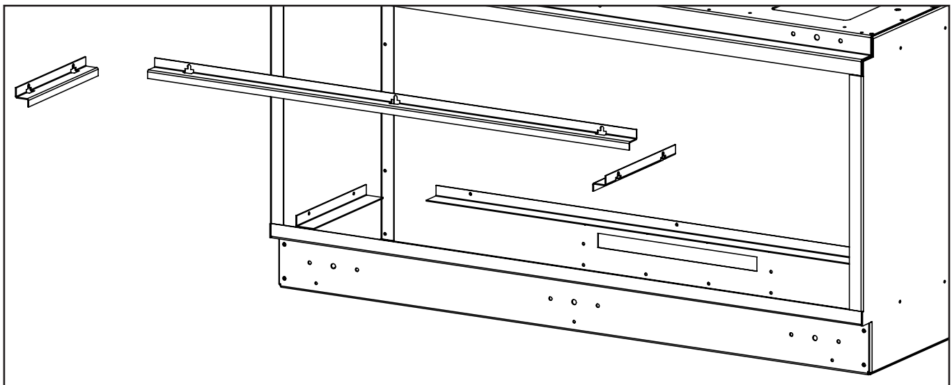
Figure 73: Panel Installation
