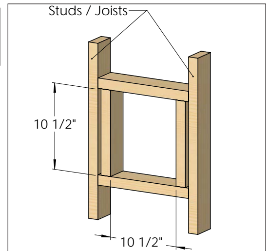
Figure 55: Vent Framing For Wall or Ceiling
