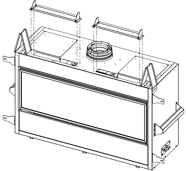
Figure 25: CSS flaps - Removal
