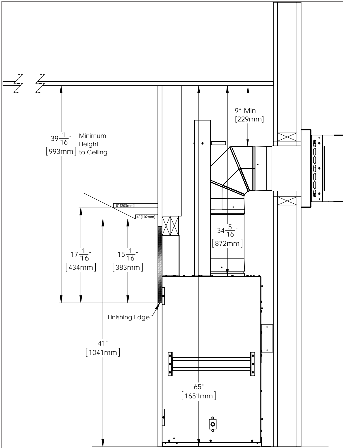
Figure 46: Install Dimensions with Mantel
