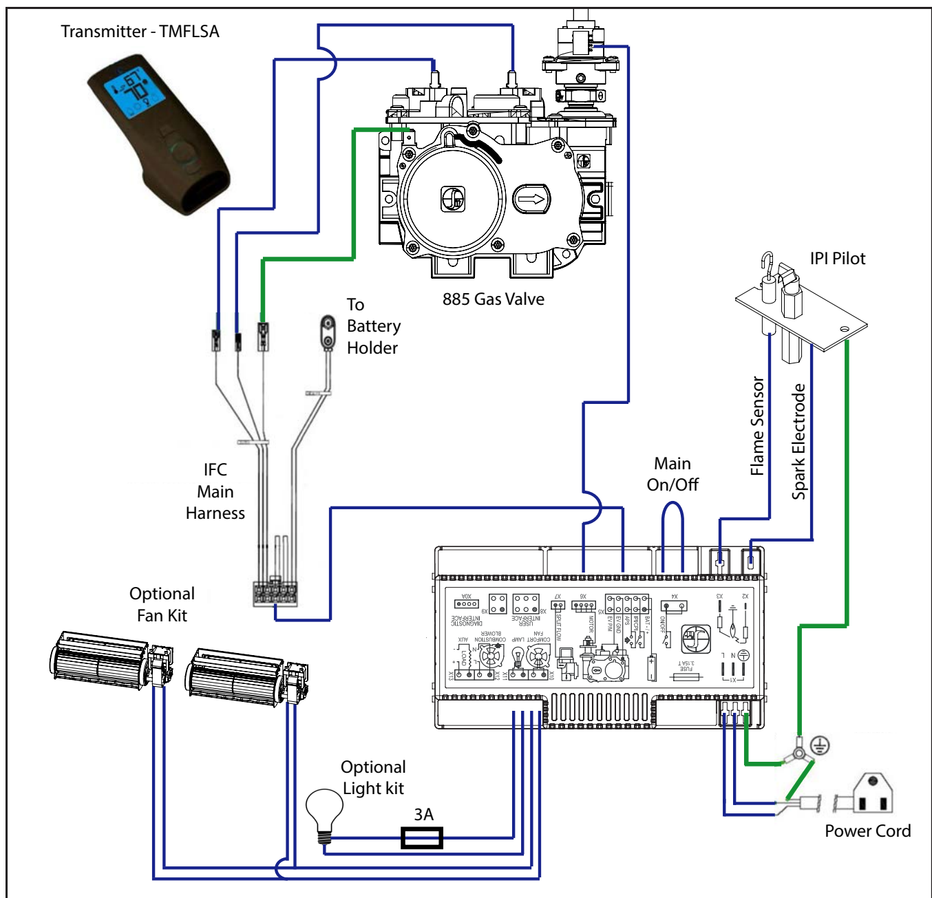
Figure 67: C34I Wiring Diagram
