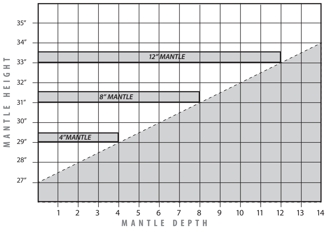
Figure 45: Minimum Mantel Height -- CSS Activated
