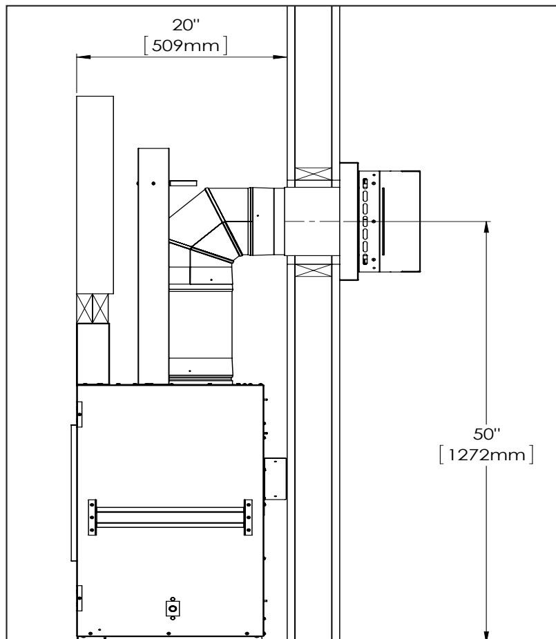
Figure 42: Minimum Horizontal Venting
