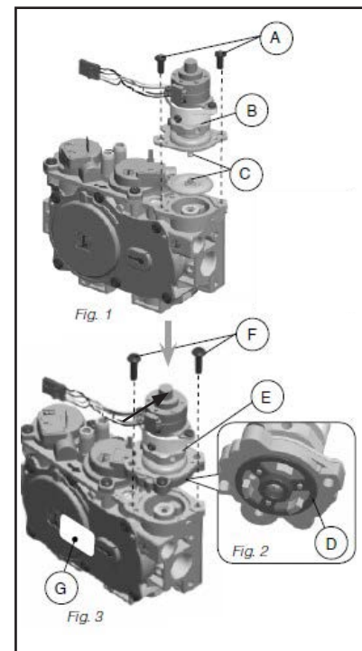
Figure 11: 885 Gas Valve
