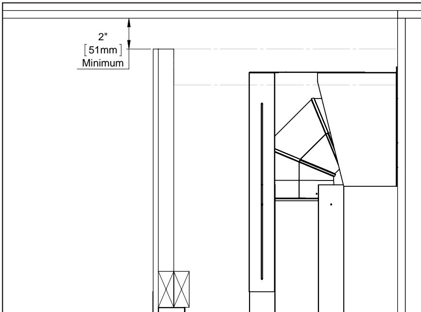
Figure 36: Open Chase
