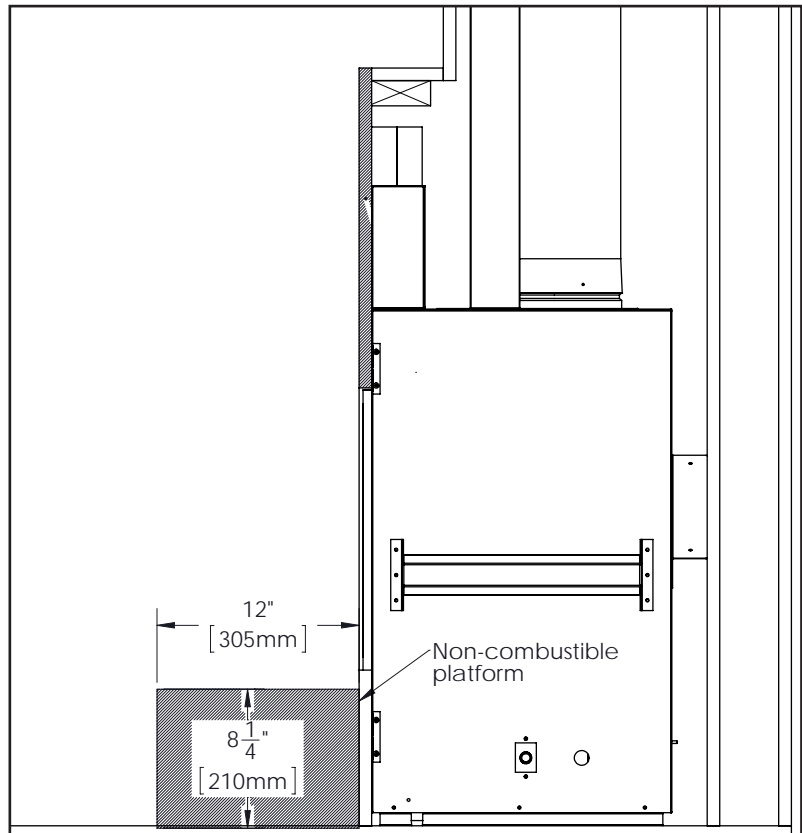
Figure 43: Non-Combustible Platform
