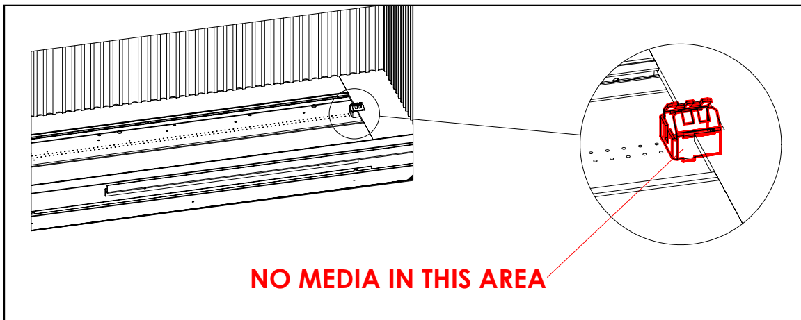
Figure 72: Protected Pilot Area
