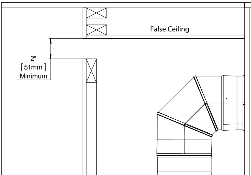
Figure 34: False Ceiling
