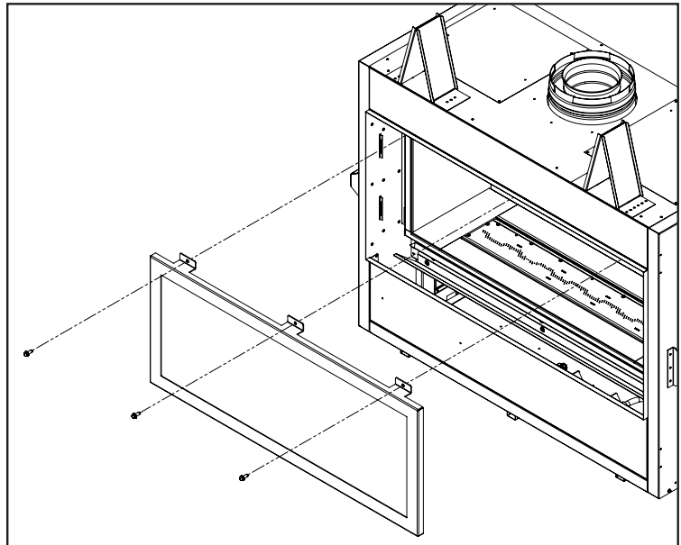
Figure 5: Door Removal Motion
