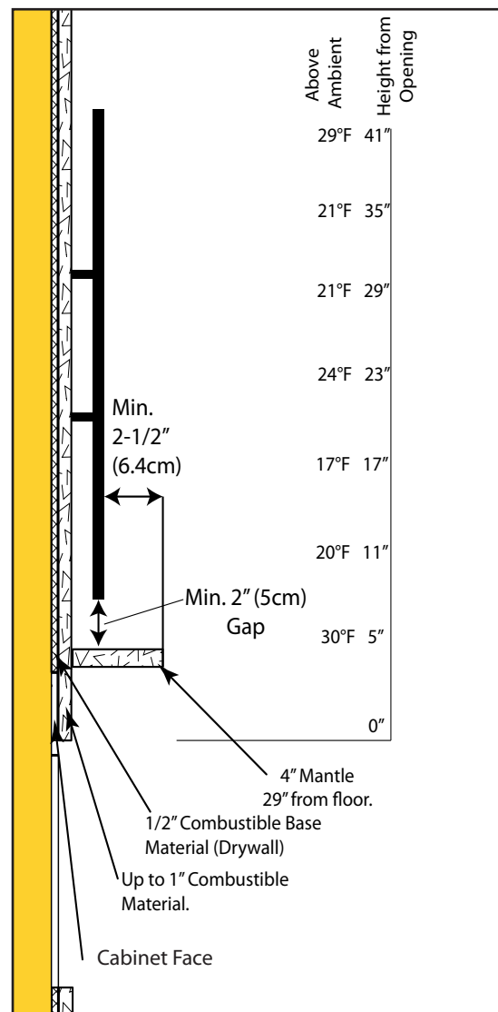
Figure 40: CSS TV Clearances
