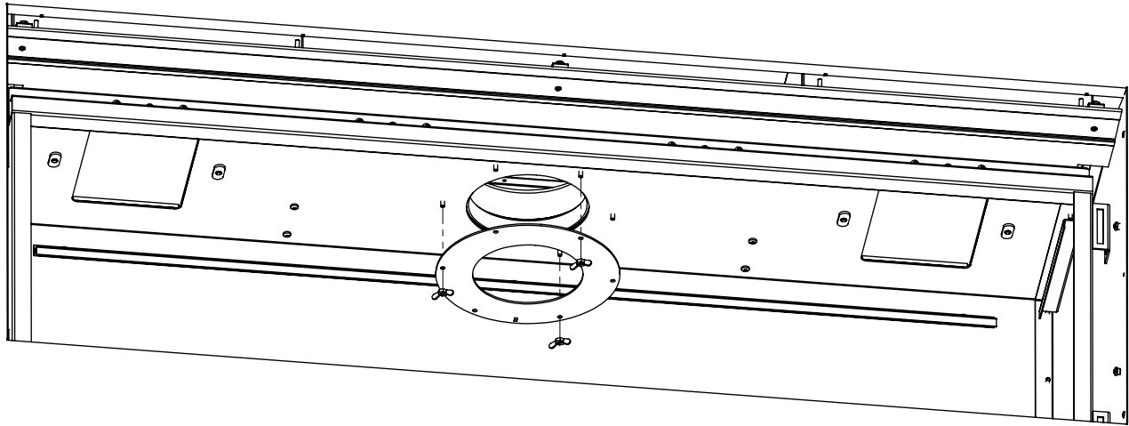
Figure 59: Restrictor Install
