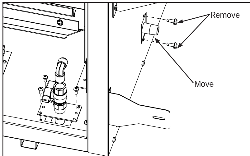
Figure 41: Alternate Gas Inlet Location
