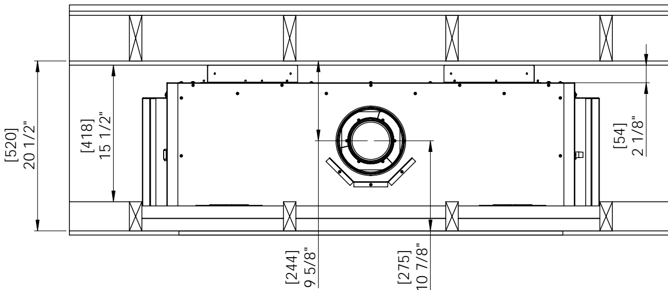
Figure 51: Dimensions for a Vertical Installation
