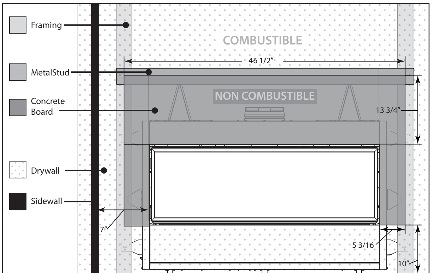
Figure 20: Finishing Non-Combustible Zone
