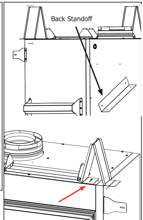
Figure 14: Fireplace Installation Prep. - 2
