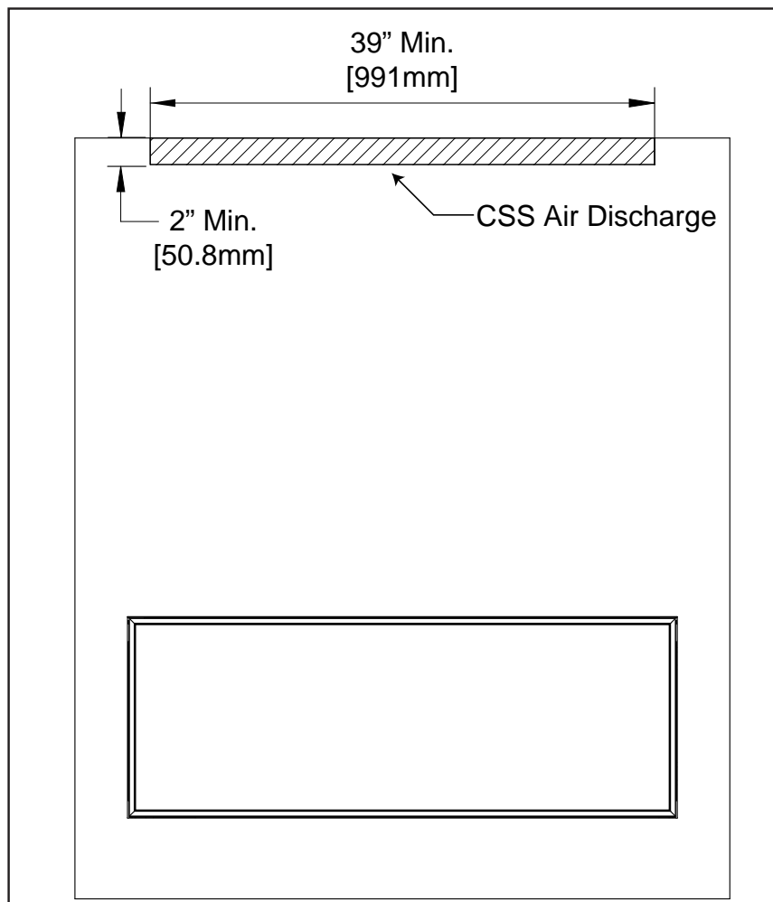
Figure 32: CSS Front Outlet
